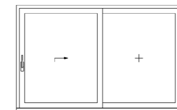
Double pane option with moving left hand and fixed right hand sash.
